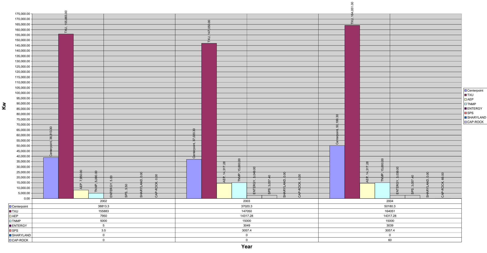
Chart TM-1 Comprehensive representation of the utilities DG activities in Texas for the calendar year 2002, 2003, and 2004
