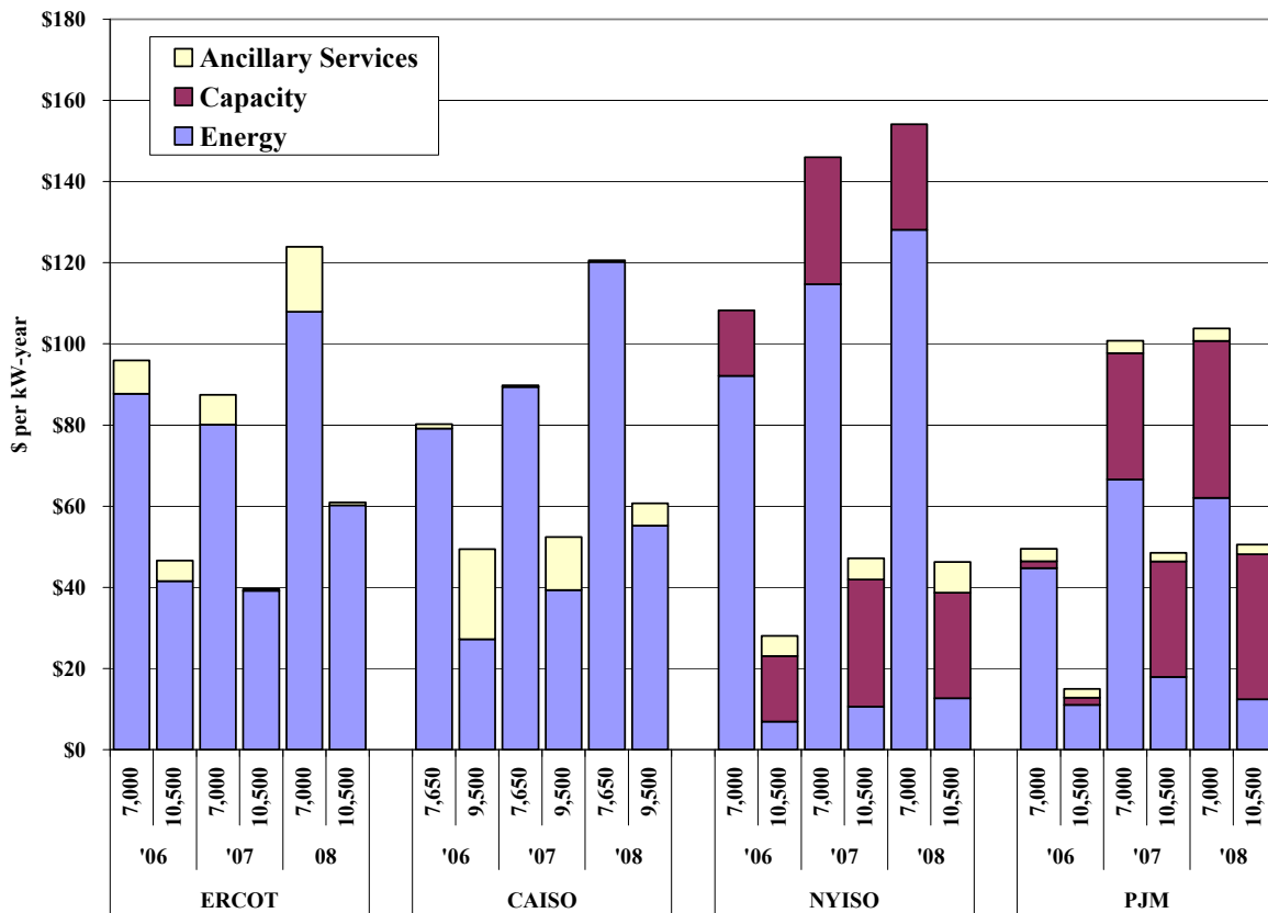
Figure 40: Comparison of Net Revenue of Gas-Fired Generation between Markets
