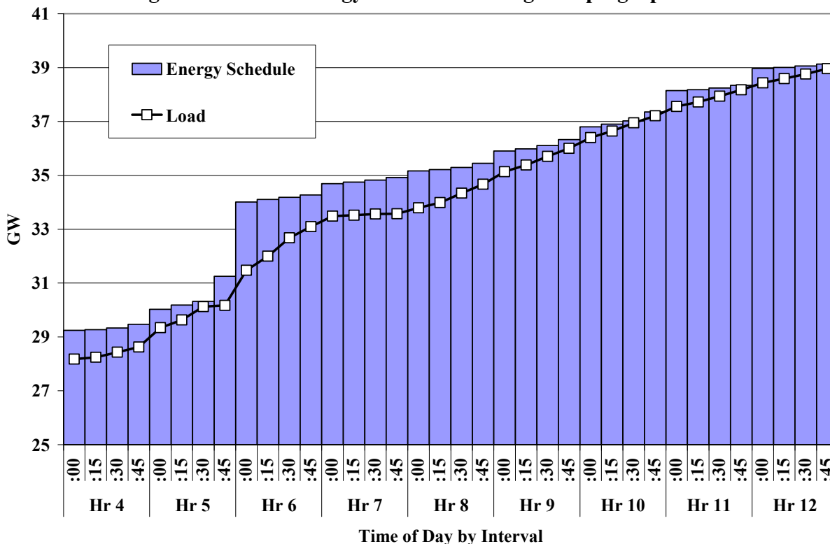
Figure 15: Final Energy Schedules during Ramping Up Hours
