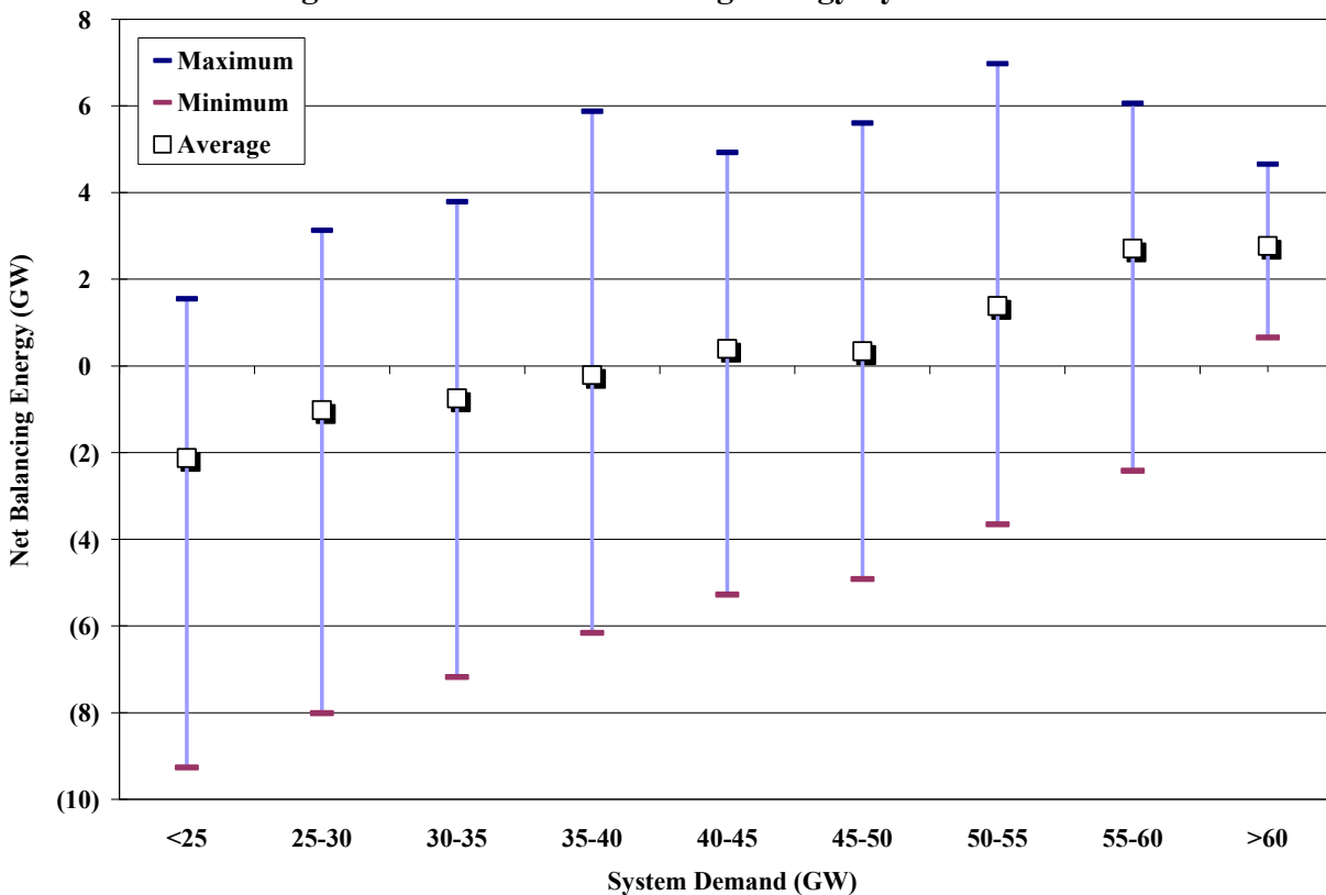
Figure 12: 2008 Net Balancing Energy by Load Level
