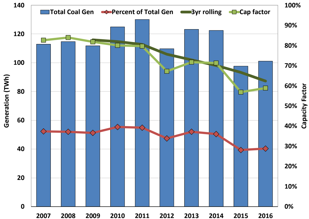
Figure 62: Historic Coal Generation and Capacity Factor
