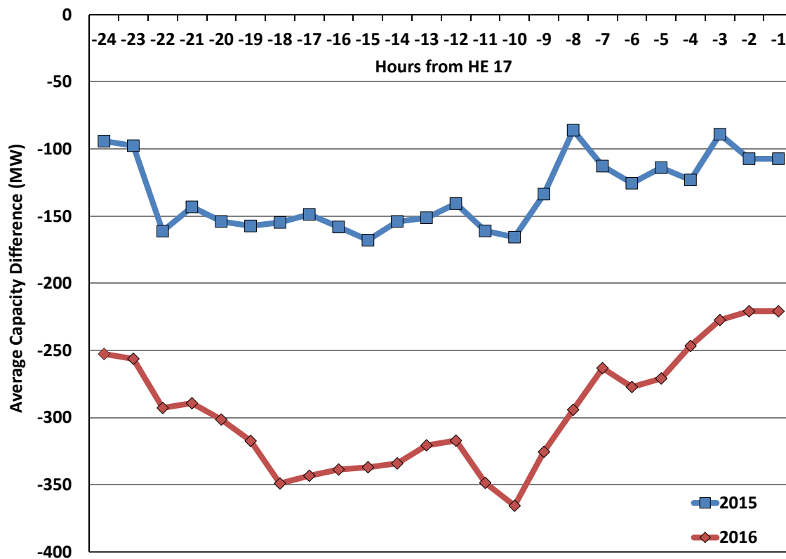
Figure 76: Capacity Commitment Timing – July and August Hour 17
