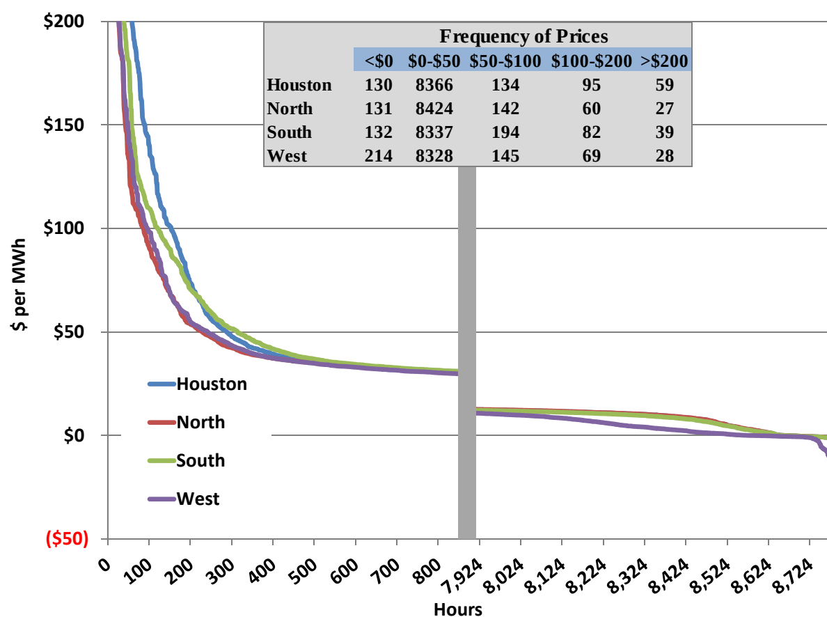
Figure 9: Zonal Price Duration Curves
