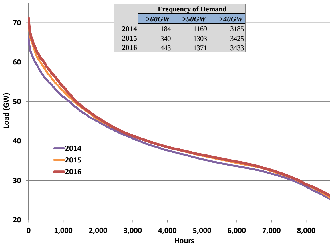
Figure 57: Load Duration Curve – All Hours
