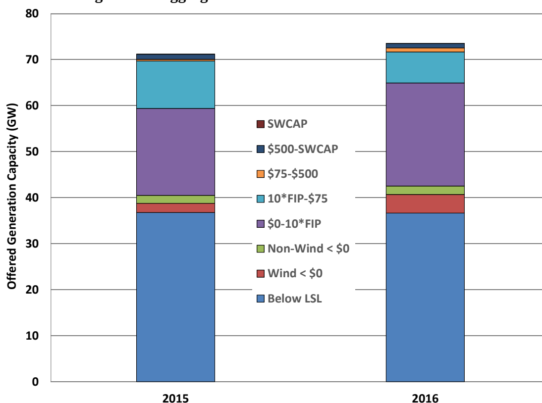
Figure 15: Aggregated Peak Hour Generation Offer Stack
